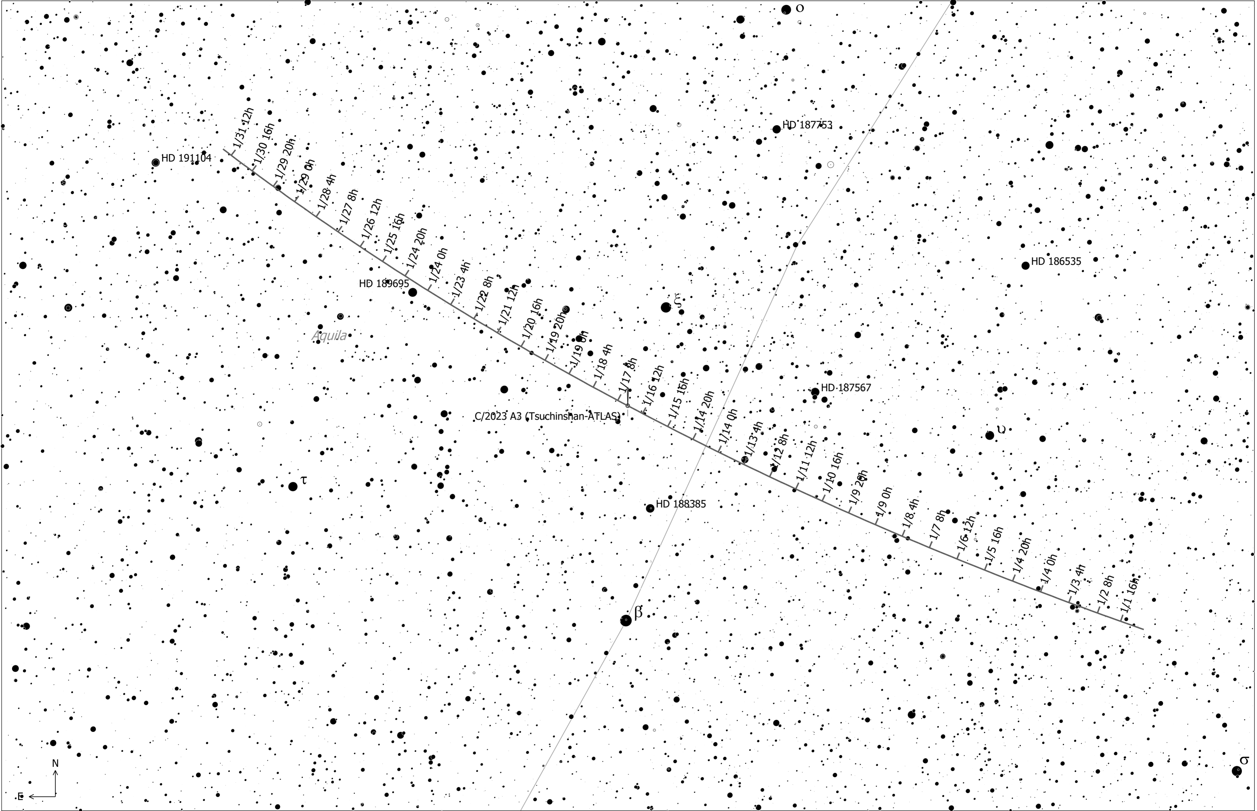
C/2023 A3 (Tsuchinshan-ATLAS) (Comet) Magnitude: 10.84 Coma Diameter: 1.5' SBr: 20.4 Mag/arcsec 2 Earth Distance: 3.0 AU
